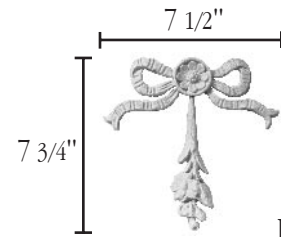
RB-001 Projection - 1/2"
